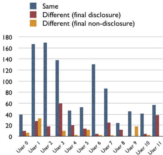
Fig. 15 Policy evolution – 12 most active target users.
