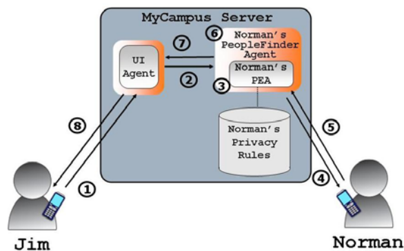
Fig. 1 Processing Jim's request for Norman's location.
