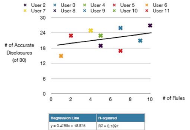
Fig. 11: Users reach a plateau: little correlation between (post-hoc) accuracy and number of rules created
