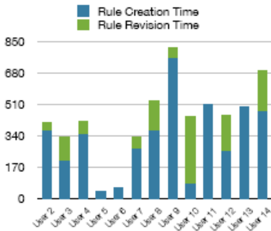
Fig. 9b Controlled lab experiments: time spent creating and modifying rules – the latter includes both changes to initial rules and addition of new rules
