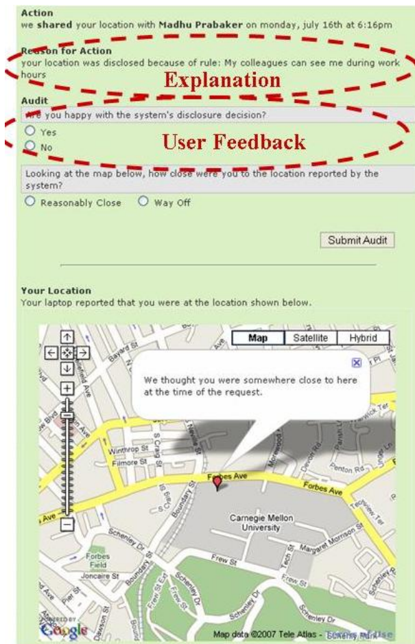
Fig. 7 Explanation can help users better understand their policies. User feedback can also be used to make suggestions or learn the user's preferences.
