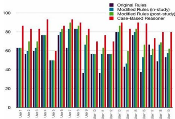
Fig. 13 User feedback can help the system learn the user’s privacy policy.
