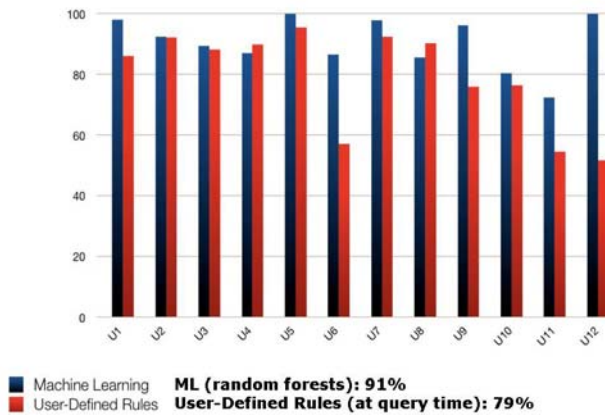
Fig. 14 Results for 12 most active target-users from 3 field pilots involving over 60 users
