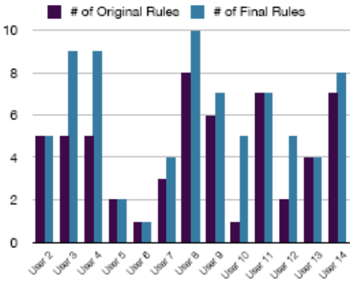
Fig. 9a Controlled lab experiments: initial number of rules versus final number of rules.
