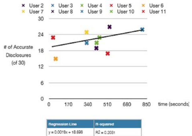
Fig. 12: Users reach a plateau: little correlation between (post-hoc) accuracy and time spent defining and refining rules.
